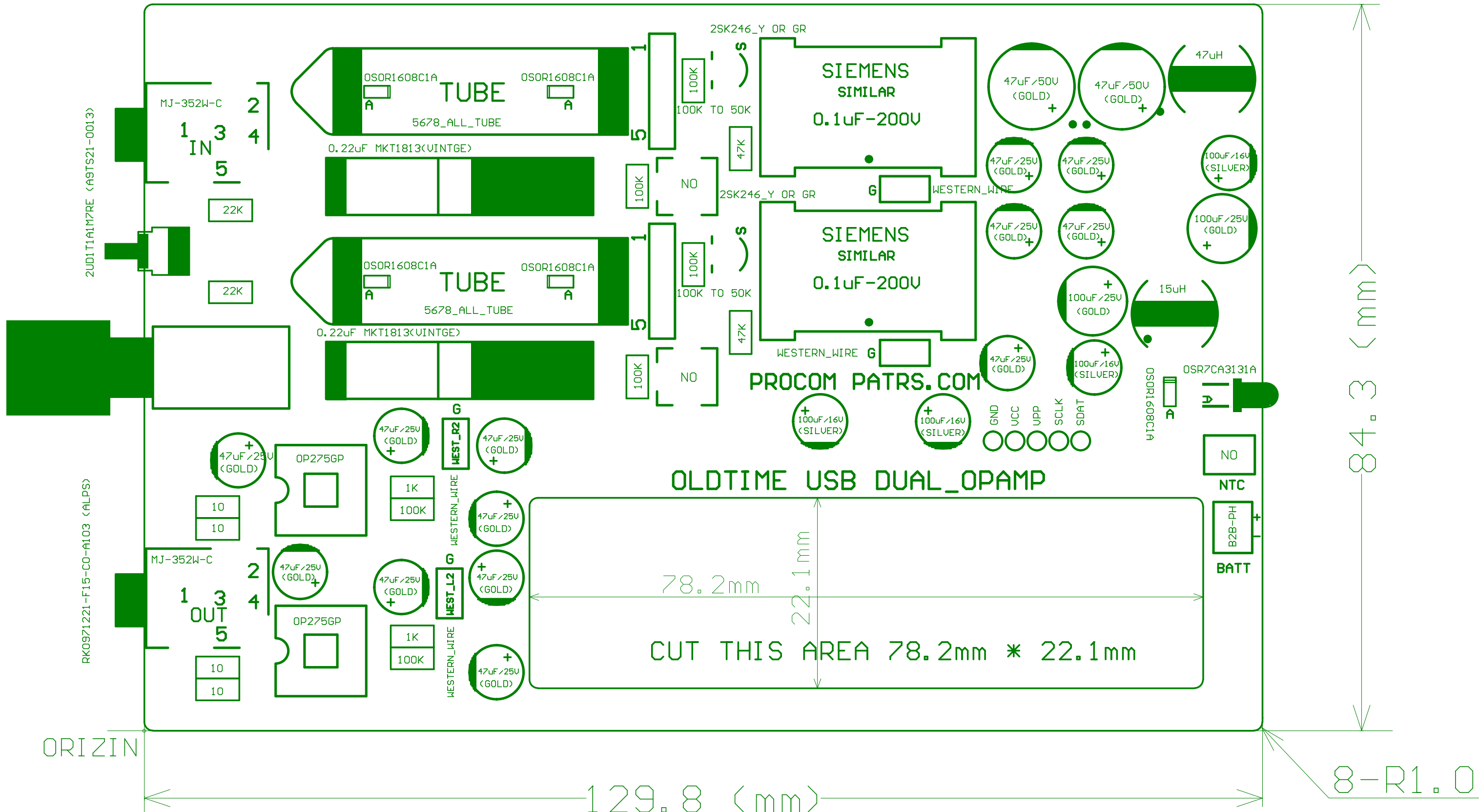
PARTS NAME DRAWING (TOP_LAYER)
